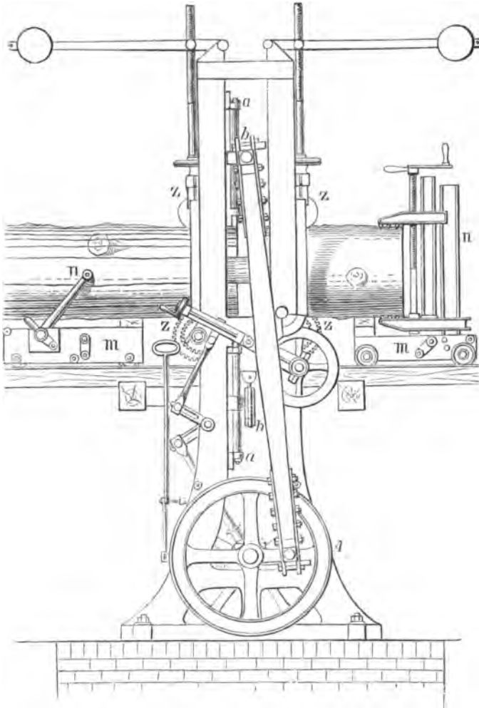
Fig. 301.—Multiple saw.
